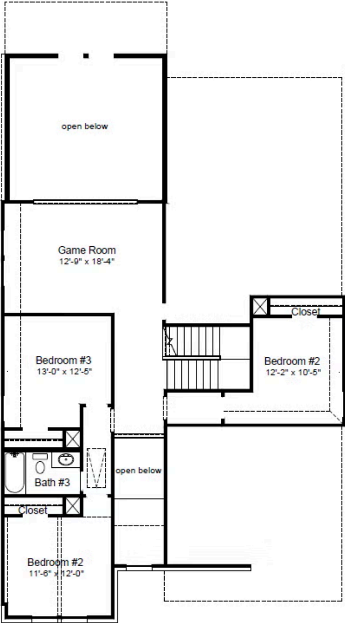
2nd Floor
