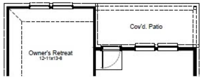
Covered Patio
