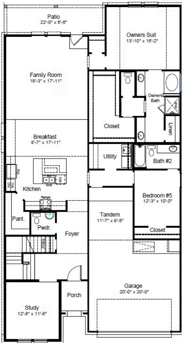
1st Floor
