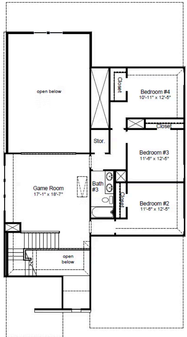
2nd Floor
