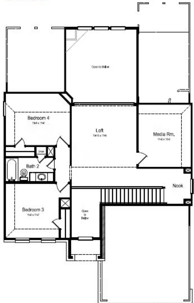
2nd Floor
