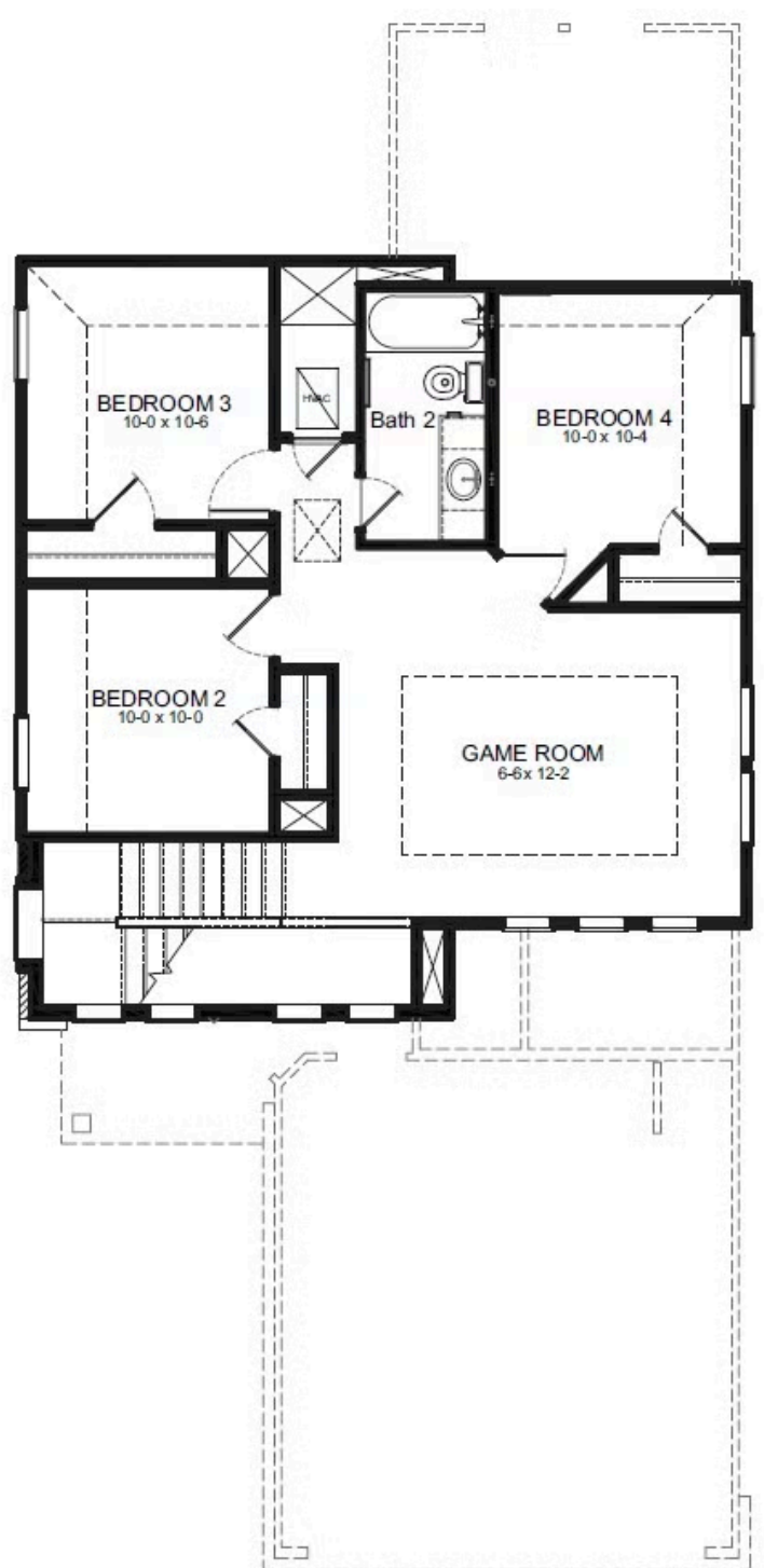
Second Floor
