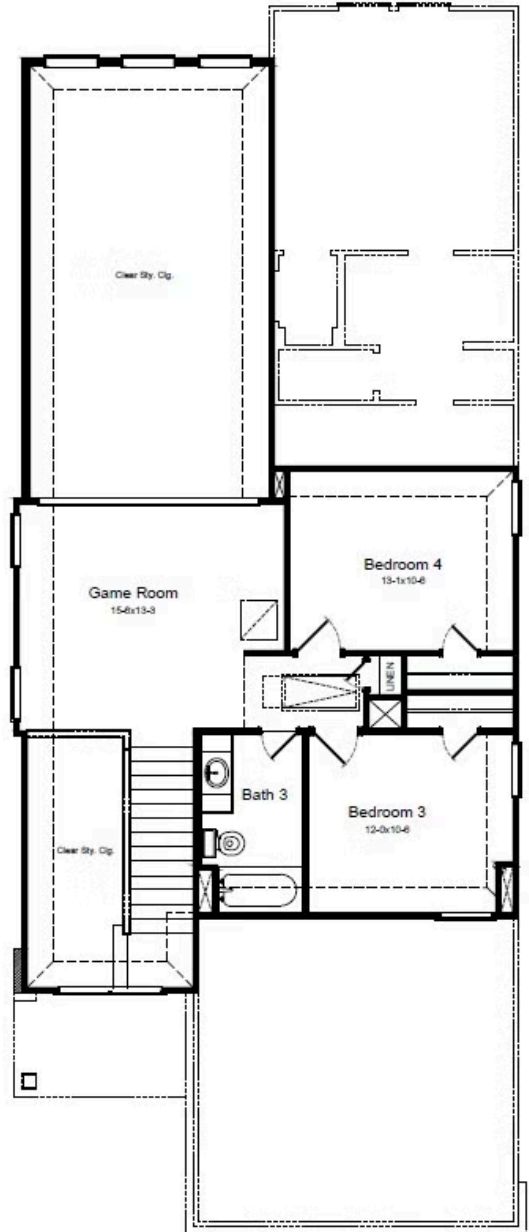
2nd Floor
