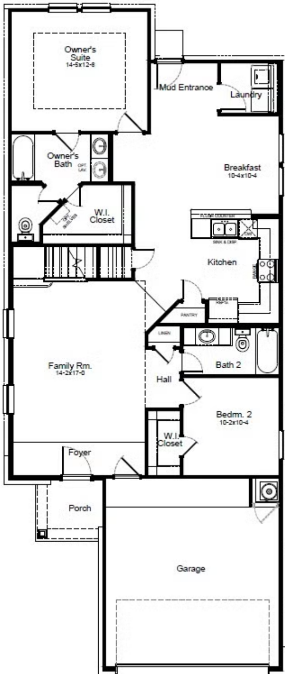
1st Floor
